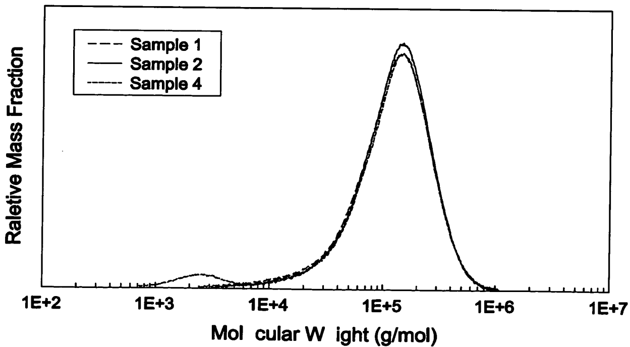
Fig. 14 Molecular Weight Distribution of Plasticized Propylene Homopolymers
